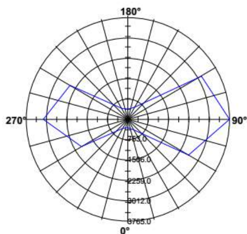
Max Plane Light Distribution Curve [Unit:cd]
